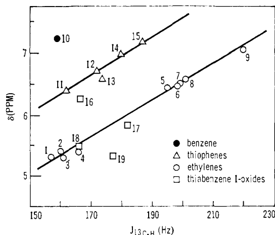
Figure 2. Plot of proton chemical shifts ( \delta ) vs. J_{^{13}\text{C}-\text{H}} values for some ethylenic compounds, thiophenes, and thiabenzene 1-oxides. All data, except those for the 1-oxides, were taken from ref 35. The compounds whose chemical shifts are plotted are as follows: (1) ethylene; (2) vinyl chloride (cis); (3) vinyl chloride (trans); (4) vinylidene chloride; (5) vinyl chloride ( \alpha ); (6) cis -dichloroethylene; (7) trans -dichloroethylene; (8) trichloroethylene; (9) vinylidene carbonate; (10) benzene; (11) 2,5-dimethylthiophene; (12) 2,5-dibromothiophene; (13) 2,5-dichlorothiophene; (14) thiophene ( \beta -H); (15) thiophene ( \alpha -H); (16) 1-methyl-3,5-diphenylthiabenzene 1-oxide ( 2a , H-4); (17) 1-methyl-3,5-diphenylthiabenzene 1-oxide ( 2a , H-2,6); (18) 1,3,5-trimethylthiabenzene 1-oxide ( 2e , H-4); and (19) 1,3,5-trimethylthiabenzene 1-oxide ( 2e , H-2,6).
