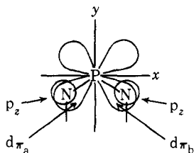
Figure 3. Dewar model for overlap in phosphonitrilic halides. The illustration shows only the upper lobes of the nitrogen 2p_z and the phosphorus d\pi_a and d\pi_b orbitals.
